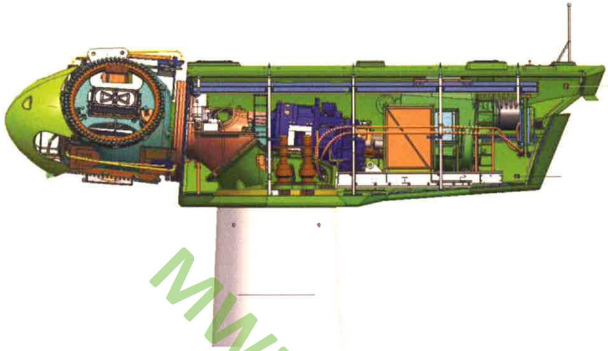
Fig. 5: 2.5-2.75 Series Nacelle
