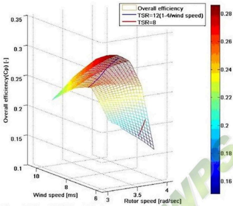
Figure 20: Overall efficiency 3-D plot
