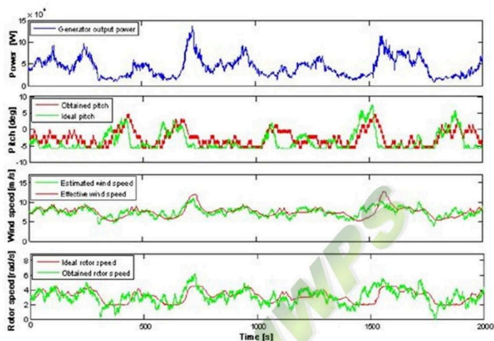
Figure 43: Speed and pitch regulator, average wind speed of 7.5 m/s
