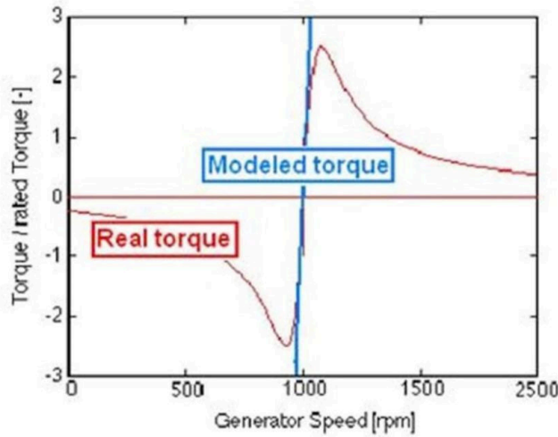
Figure 6: Generator torque vs. speed
