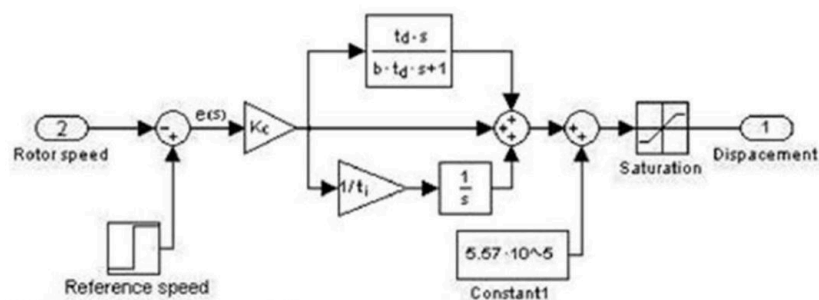
Figure 28: P, PI, PID controller
