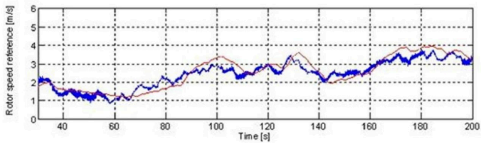
Figure 39: Rotor speed reference
