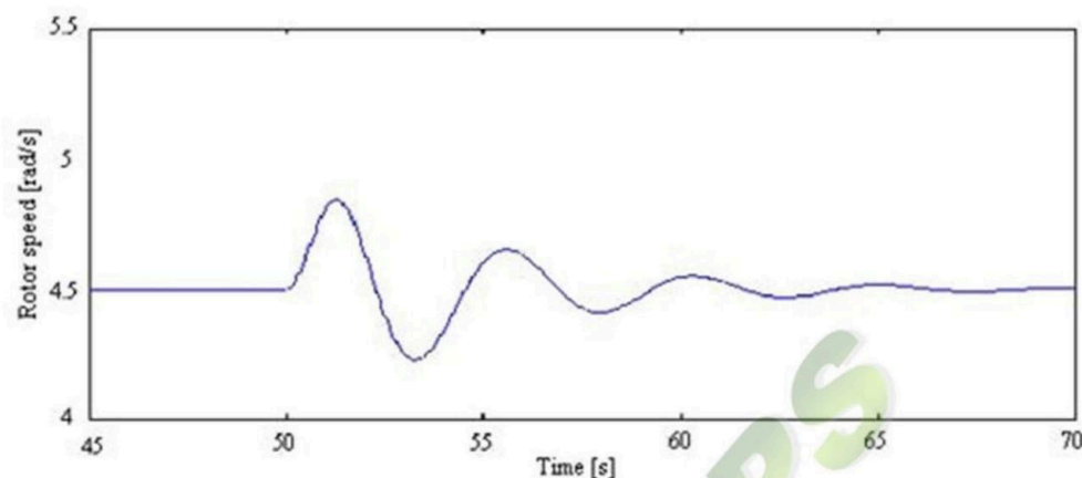
Figure 33: Rotor speed wind step response
